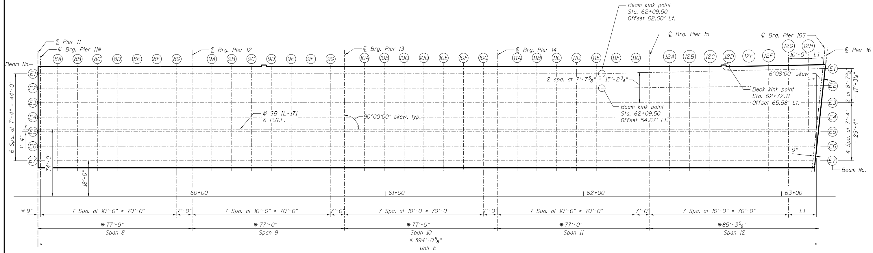
PLAN - UNIT E
