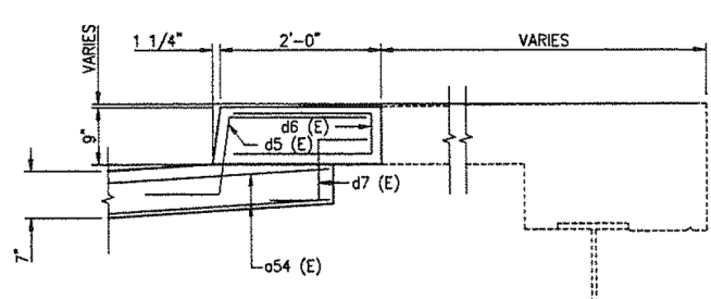
MEDIAN SECTION
