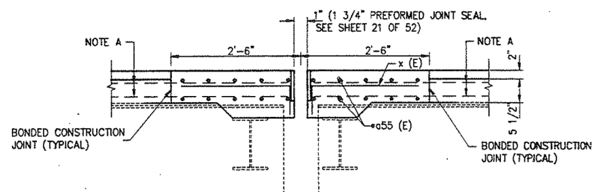
SECTION H-H PROPOSED NOTE: REINFORCEMENT IS SAME BOTH SIDES OF JOINT
