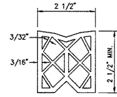
PREFORMED JOINT SEAL (2 1/2")
