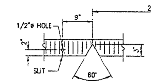
SEAL CUT-OUT @ CURB
