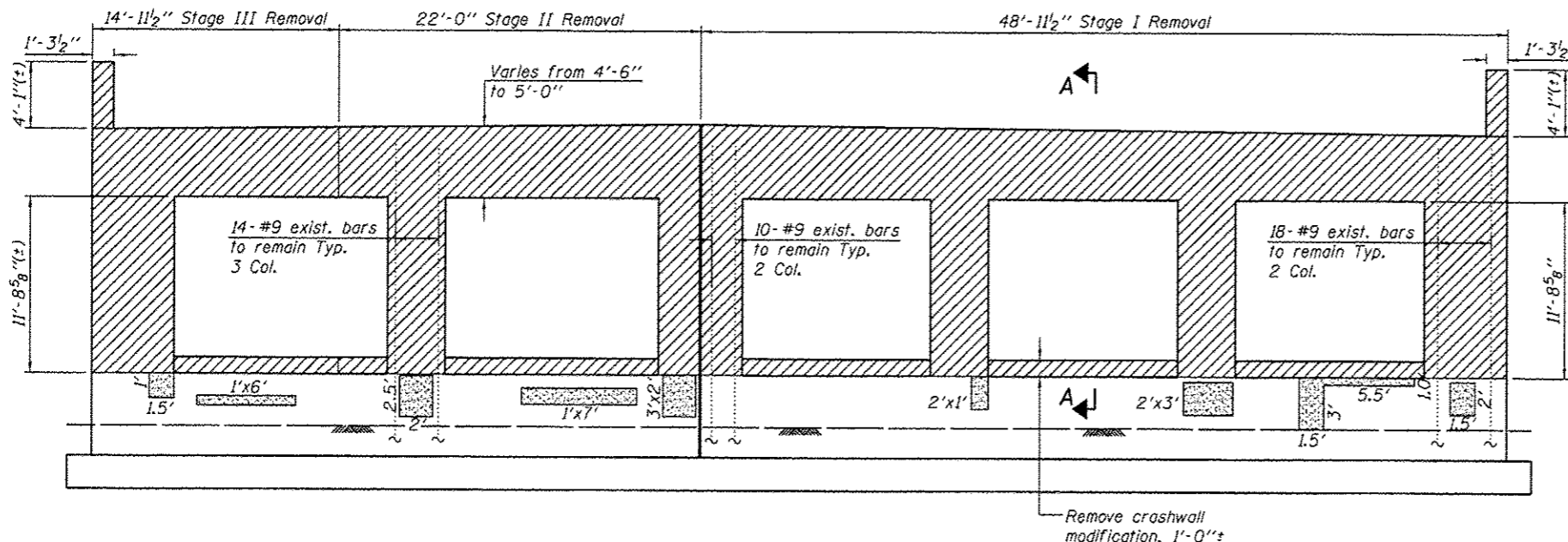
PIER 1 ELEVATION (Looking East)
