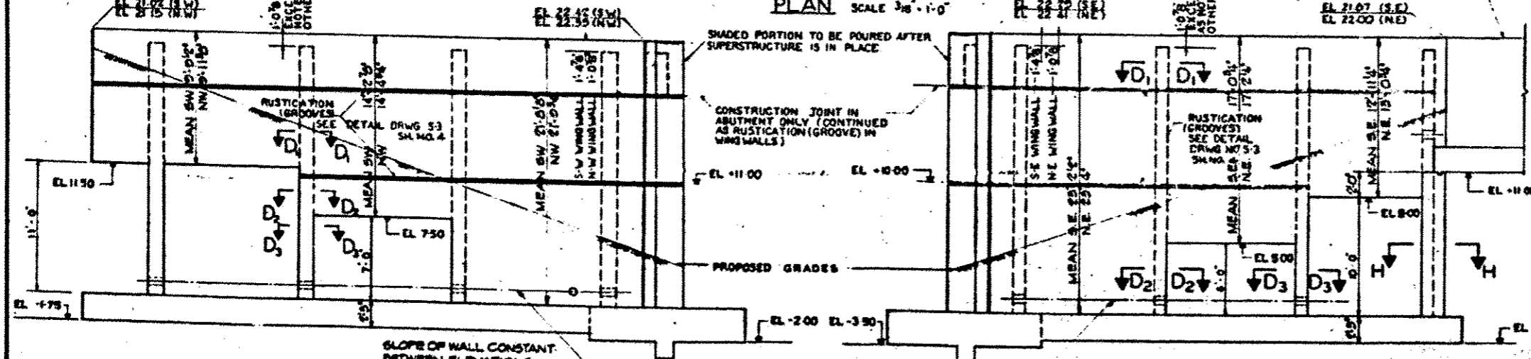
ELEVATION S-W WING WALL SCALE 3/8" = 1'-0" N-W WING WALL (SIMILAR EXCEPT WHERE NOTED)
