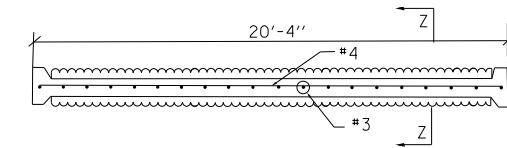
TYPICAL WALL PLAN
