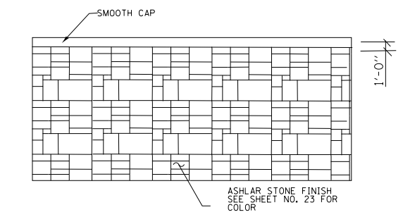
TYPICAL PANEL DETAIL W/ FINISH
