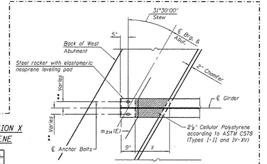
PARTIAL PLAN AT WEST ABUTMENT (Showing bottom flange of girder)
