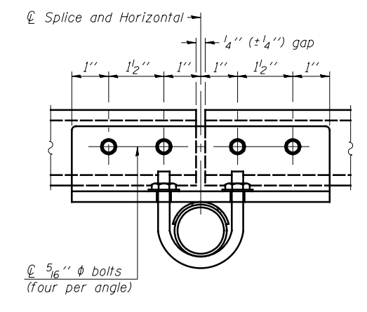
SECTION T-T
