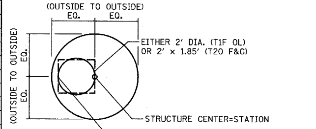
CATCH BASIN (PRECAST REINFORCED CONCRETE SECTION)
