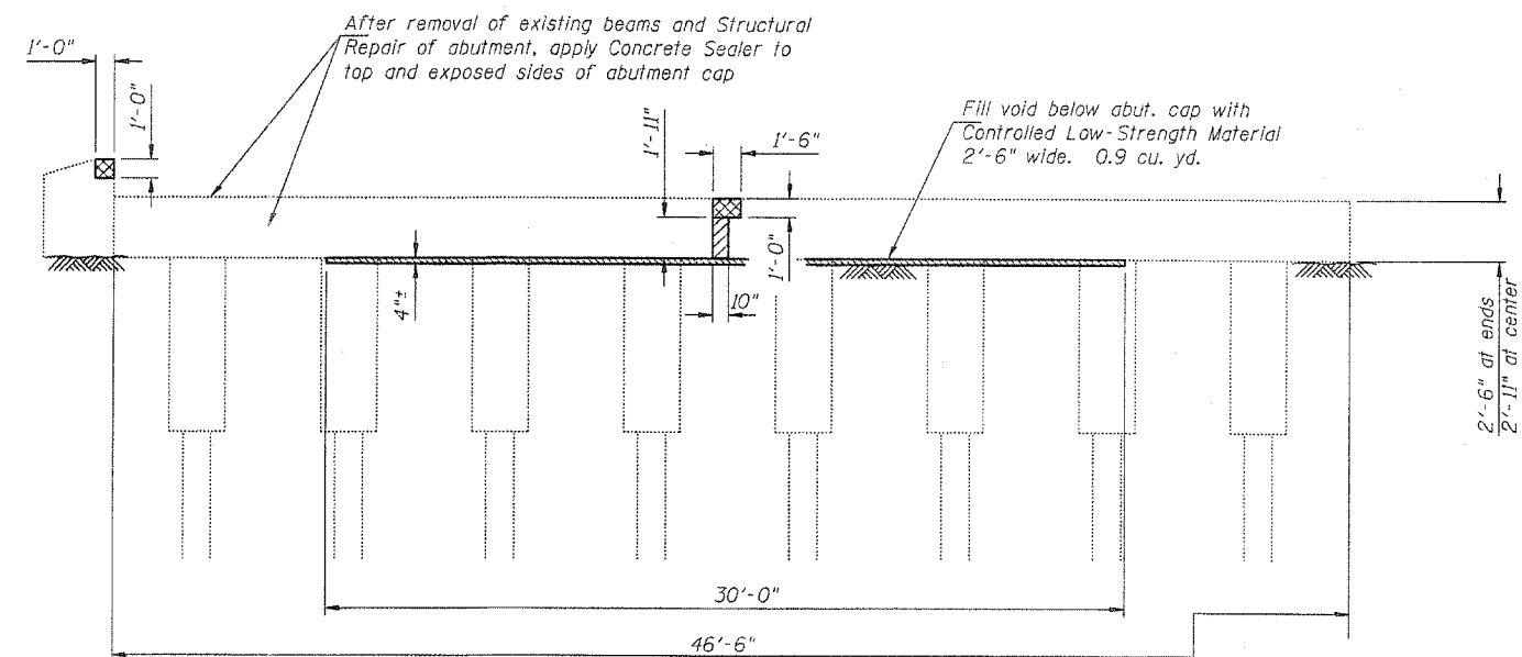
SOUTH ABUTMENT
