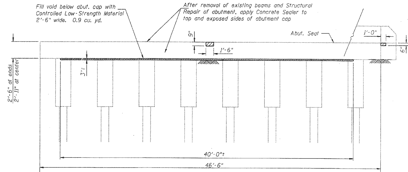
NORTH ABUTMENT
