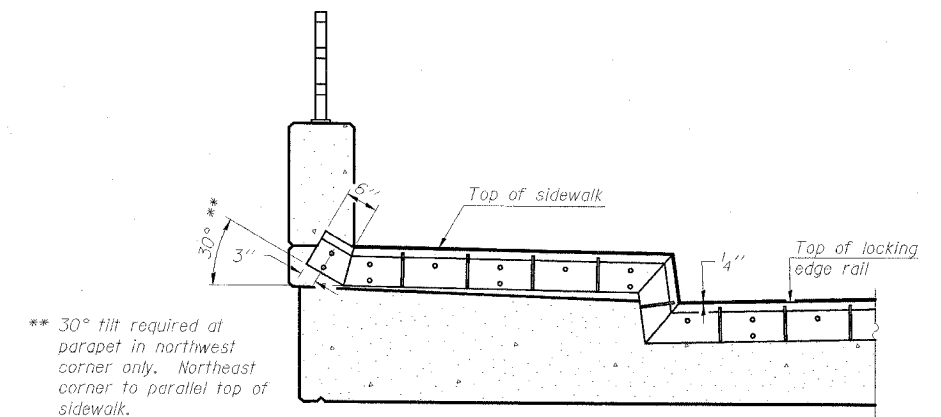
END TREATMENT AT SIDEWALK
