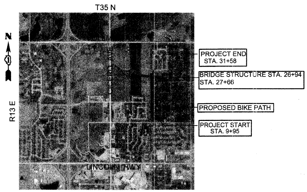
LOCATION MAP PROJECT LENGTH 2163.00 FT (0.4097 MILES)
