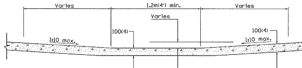
SEC. B-B
