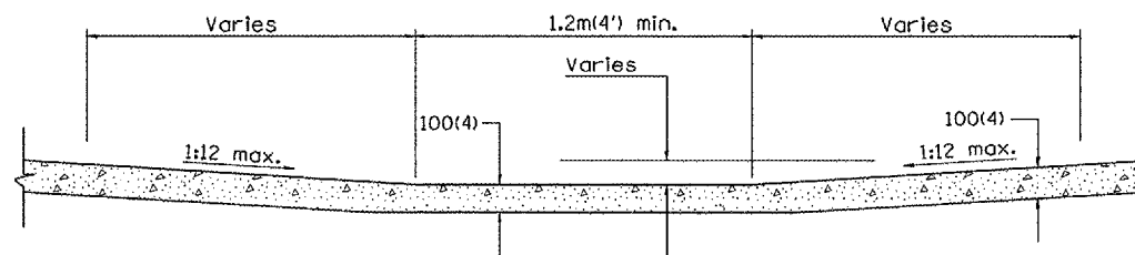
SEC. D-D
