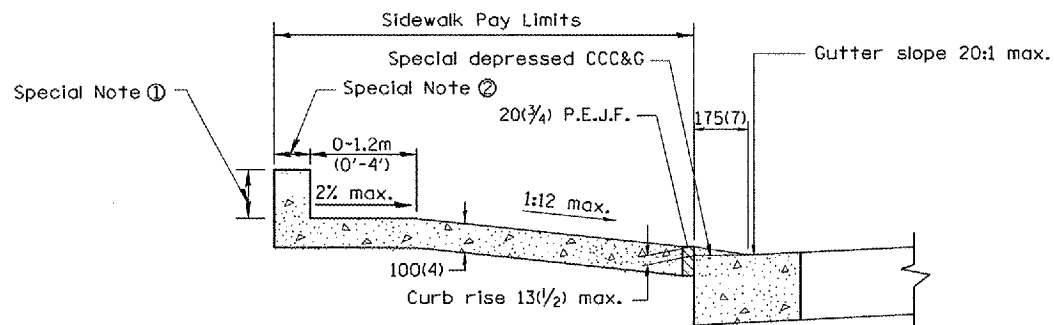
SEC. C-C
