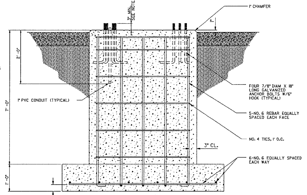
ELEVATION SECTION B
