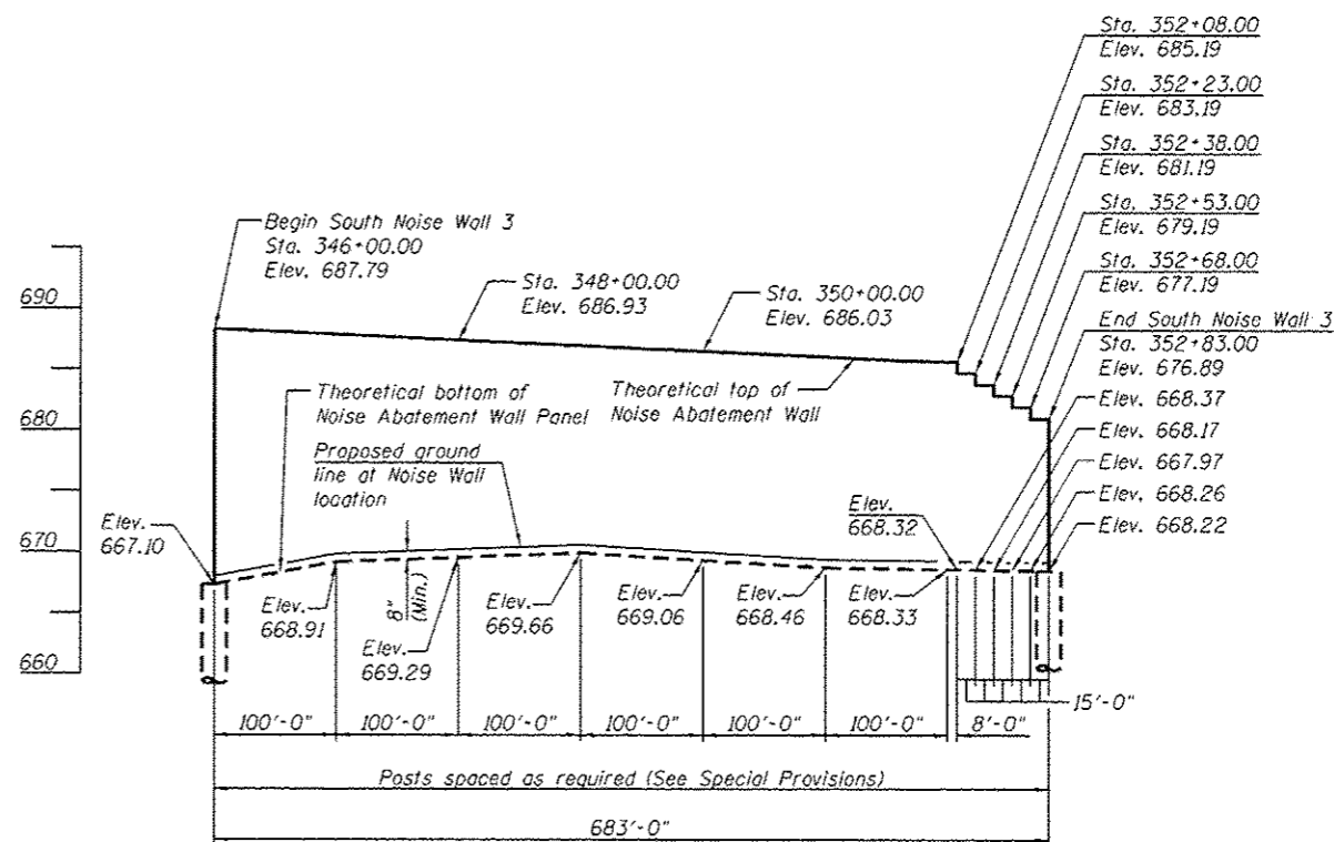
SOUTH NOISE ABATEMENT WALL 3 ELEVATION (Looking North)
