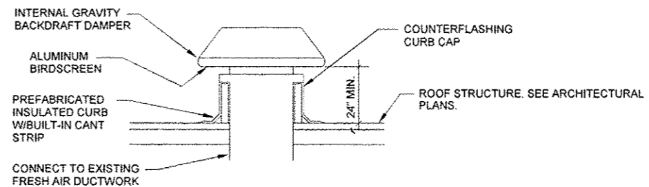
2 ROOF MOUNTED INTAKE VENTILATOR DETAIL N.T.S.
