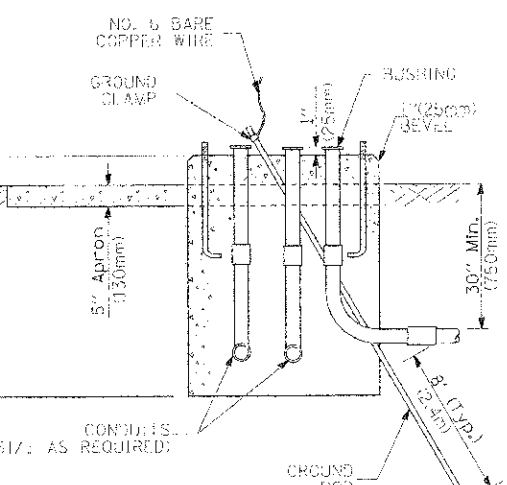
TYPE D FOR GROUND MOUNTED CONTROLLER CABINET AND UPS BATTERY CABINET
