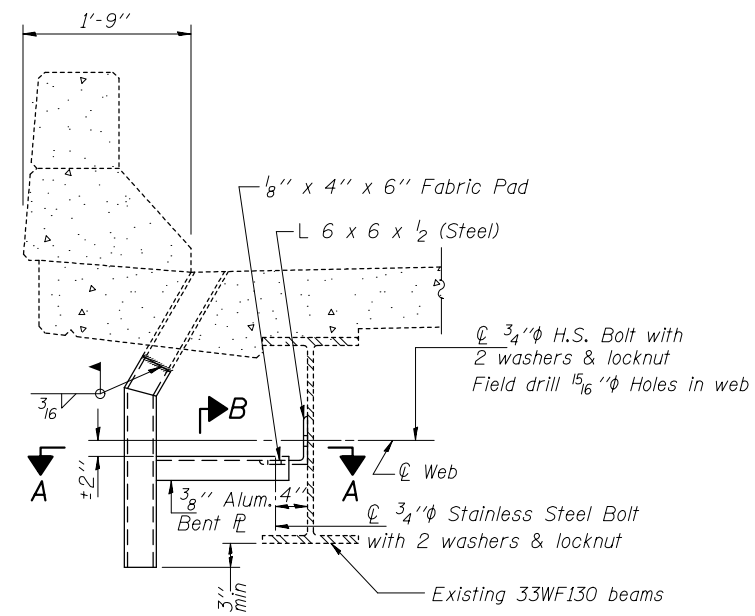
SECTION AT DRAIN
