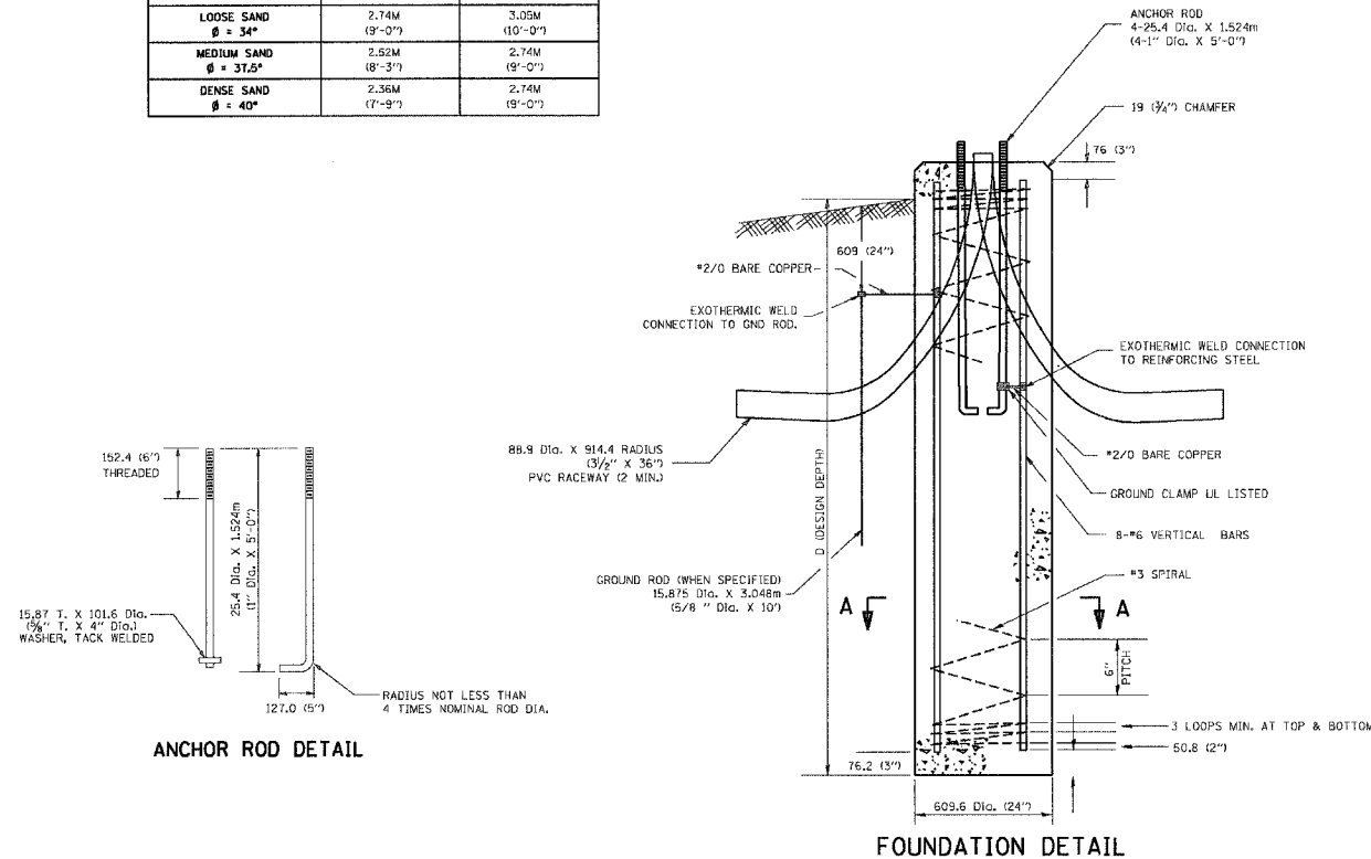
FOUNDATION DETAIL
