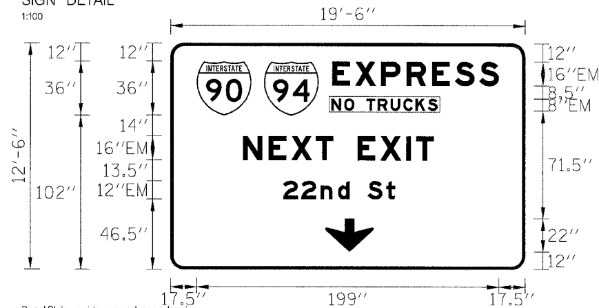
SIGN DETAIL 1:100
