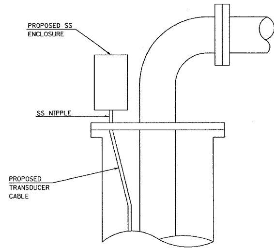
WELL HEAD DETAIL
