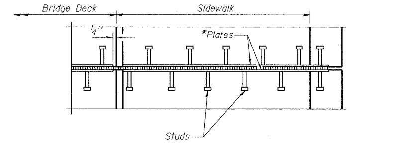
PLAN AT SIDEWALK
