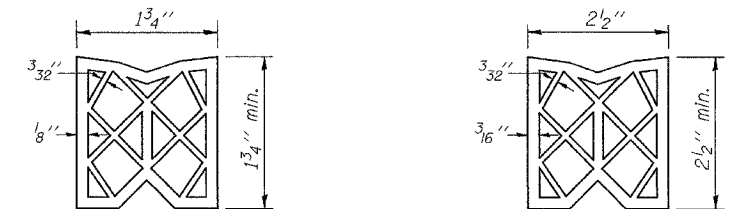
PREFORMED JOINT SEAL (1 3/4") PREFORMED JOINT SEAL (2 1/2")
