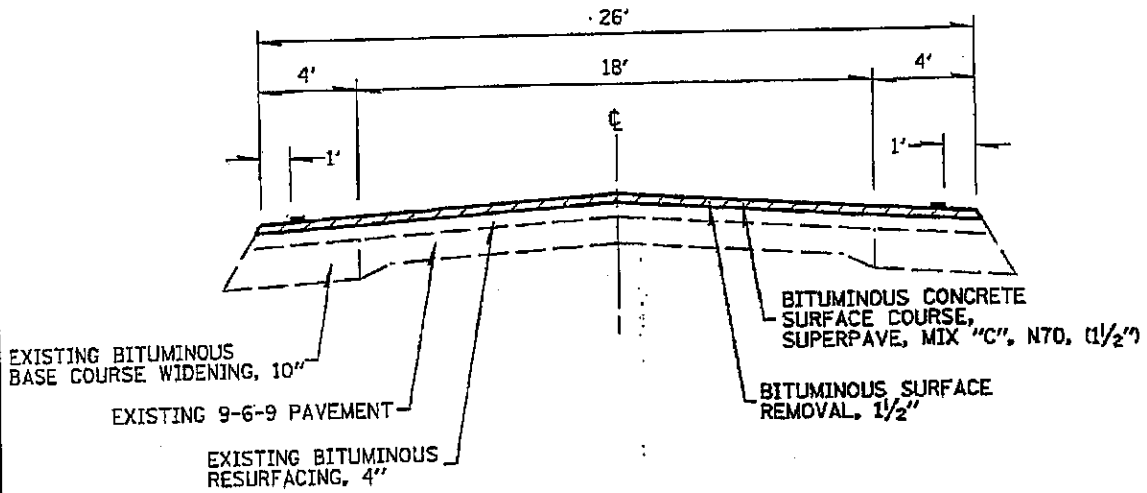
TYPICAL SECTION
