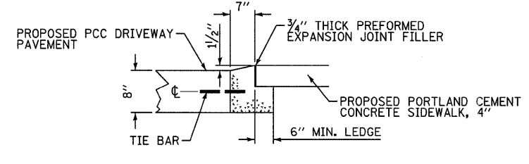
SECTION C-C ADJACENT TO SIDEWALK
