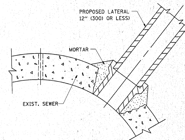
DETAIL "C"
