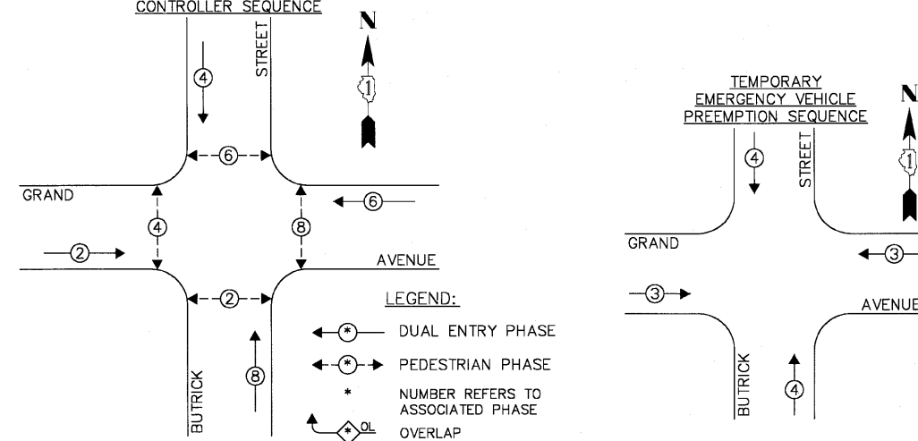
TEMPORARY PHASE DESIGNATION DIAGRAM
