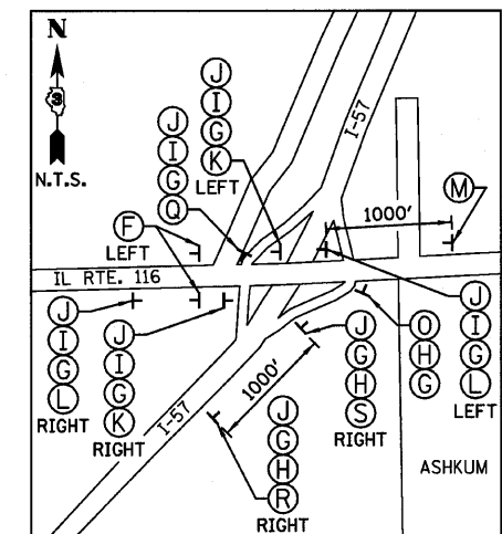
VILLAGE OF ASHKUM INTERCHANGE (DETAIL "D")
