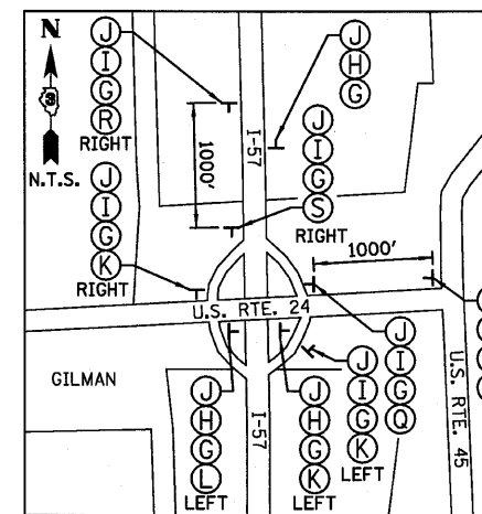
CITY OF GILMAN INTERCHANGE (DETAIL "C")
