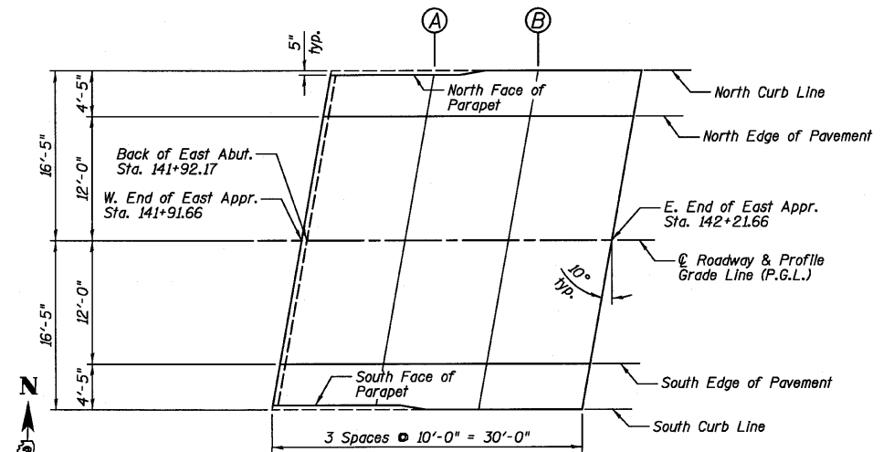
EAST APPROACH SLAB PLAN
