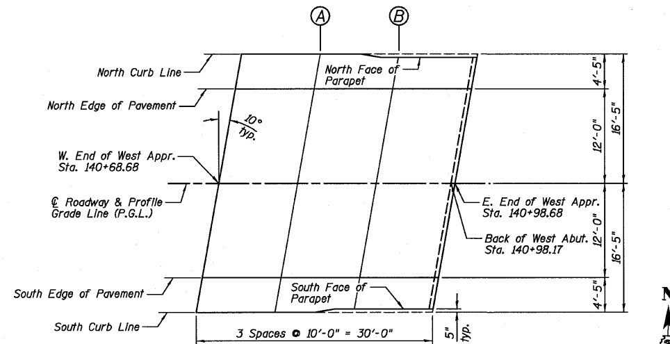
WEST APPROACH SLAB PLAN
