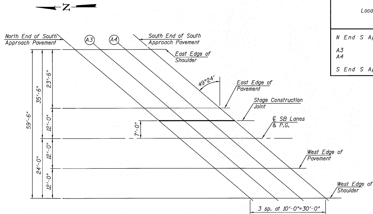
PLAN S. Approach (SB)
