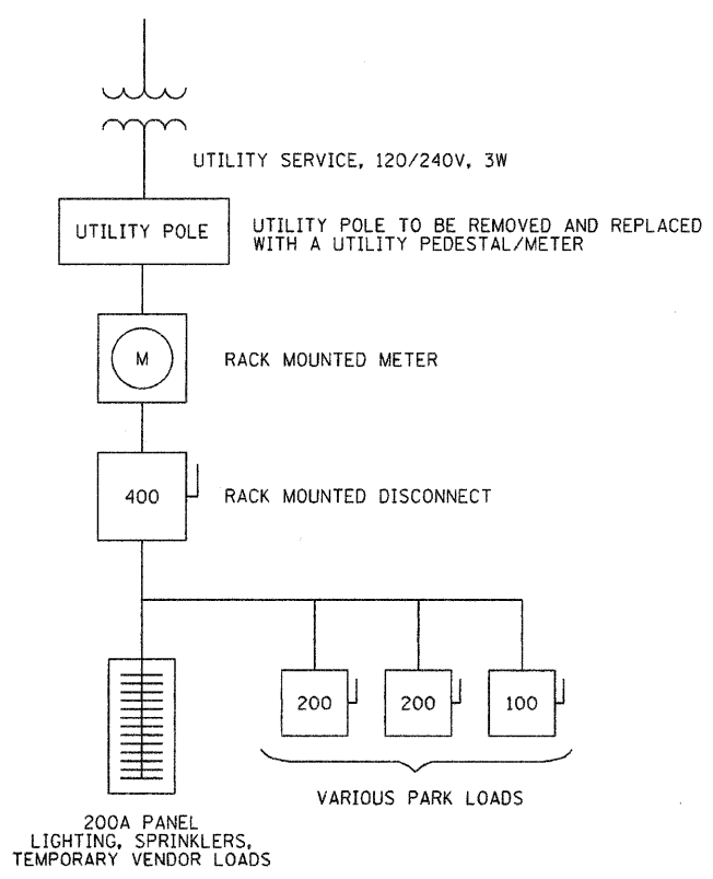
EXISTING ONE LINE
