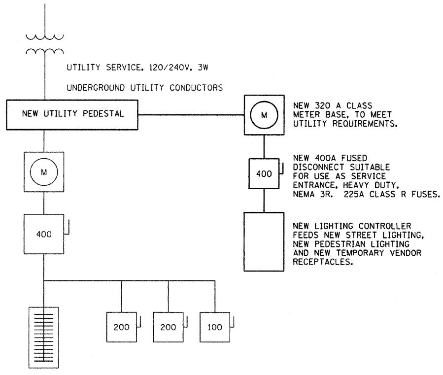
NEW ONE LINE (NEW EQUIPMENT IN BOLD)
