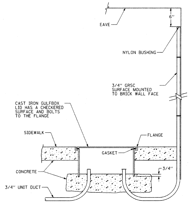
SIDEWALK GULFBBOX DETAIL
