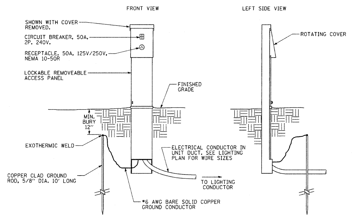
POWER PEDESTAL DETAIL (TYP. OF 4, SEE LIGHTING LAYOUT PLAN)
