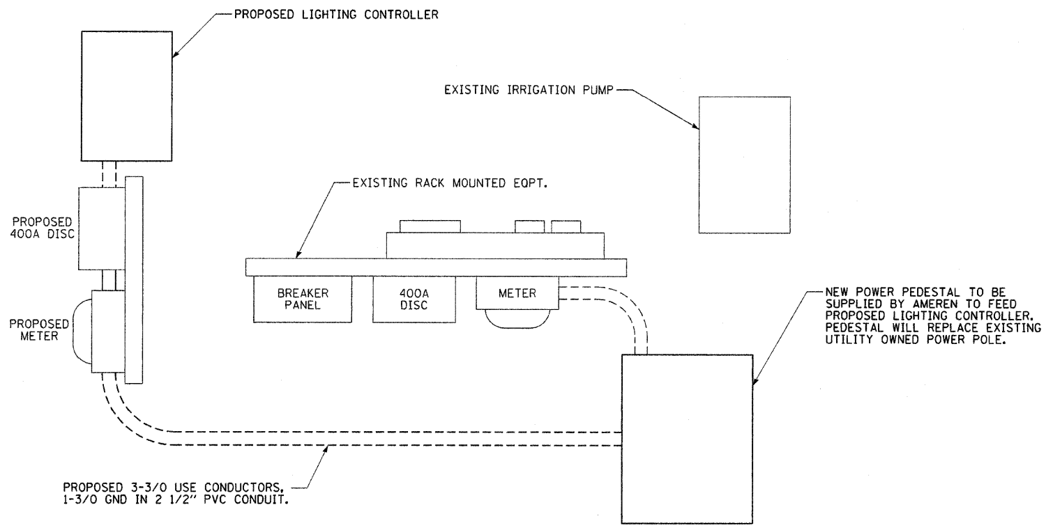
PROPOSED LIGHTING CONTROLLER AND UTILITY PEDESTAL (N.T.S.)
