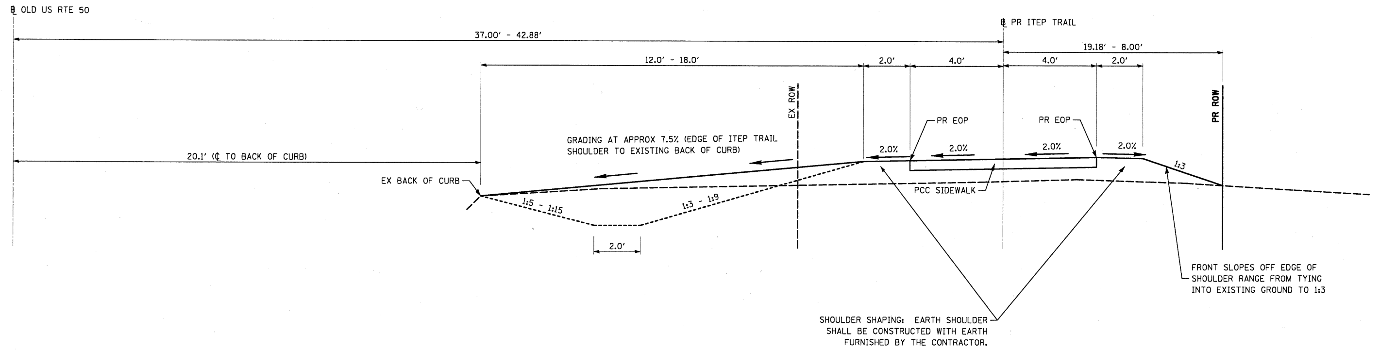
PROPOSED TYPICAL SECTION STA 13+88 TO STA 15+75 (2.0' DITCH) STA 15+75 TO STA 17+85 (GRADED TO DRAIN TO BACK OF CURB)
