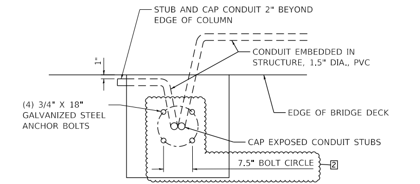
PLAN VIEW AT COLUMN AT WEST ABUTMENT (EAST ABUTMENT IS MIRRORED)
