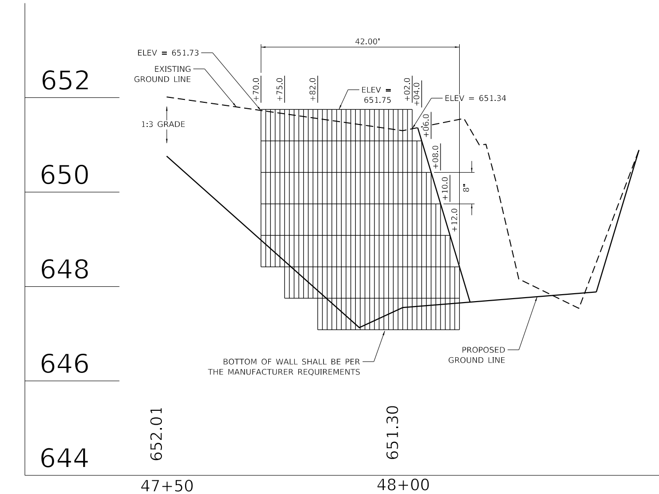
SEGMENTAL CONCRETE BLOCK WALL DETAIL 5
