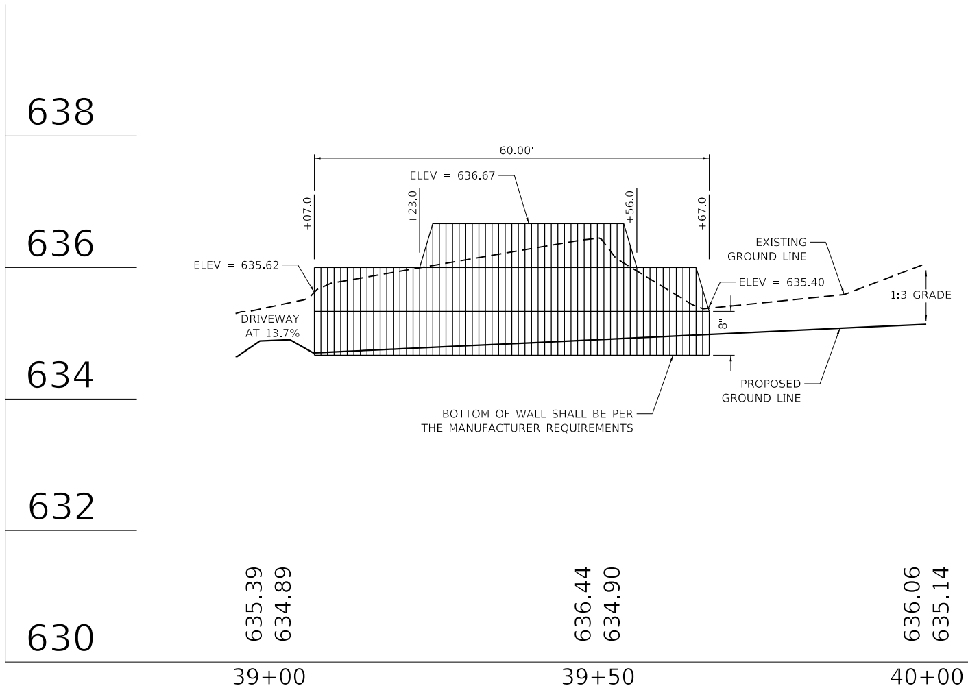
SEGMENTAL CONCRETE BLOCK WALL DETAIL 3
