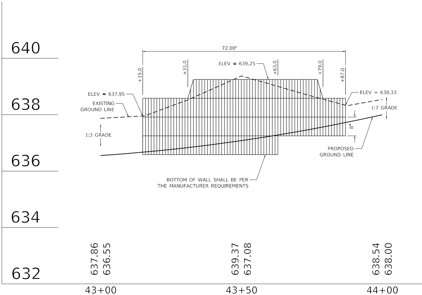
SEGMENTAL CONCRETE BLOCK WALL DETAIL 4
