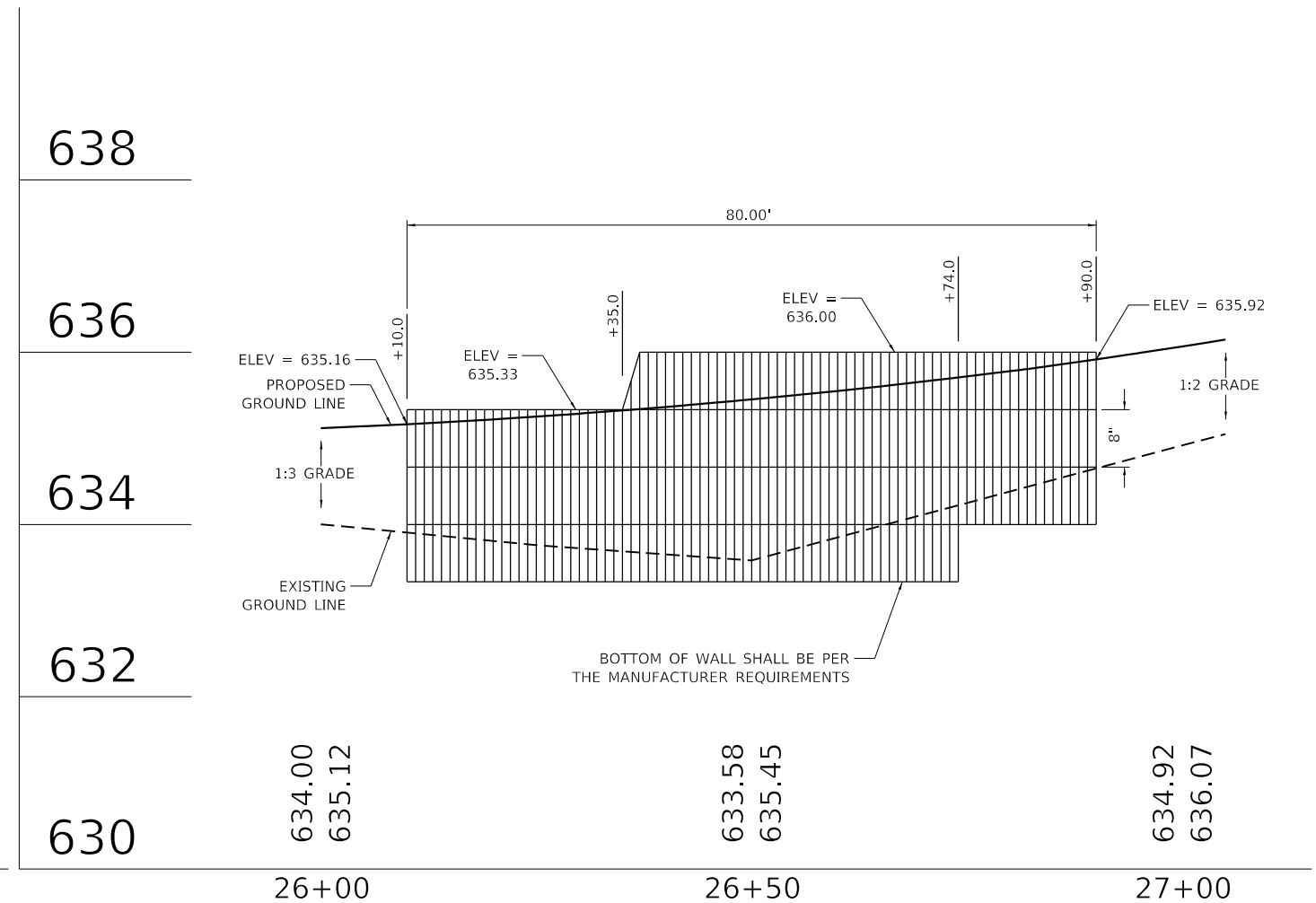
SEGMENTAL CONCRETE BLOCK WALL DETAIL 2
