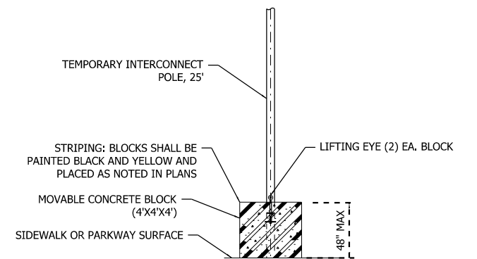
PORTABLE TEMPORARY POLE, 25' NOT TO SCALE
