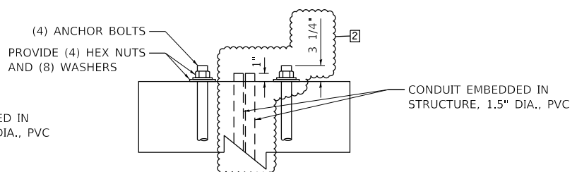
ELEVATION VIEW AT COLUMN (NOT TO SCALE)
