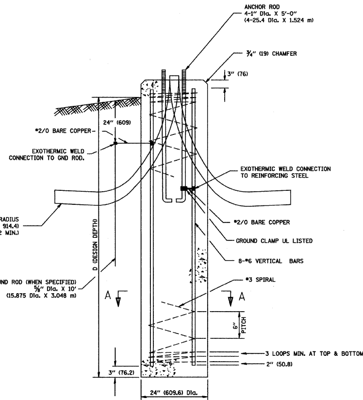
FOUNDATION DETAIL
