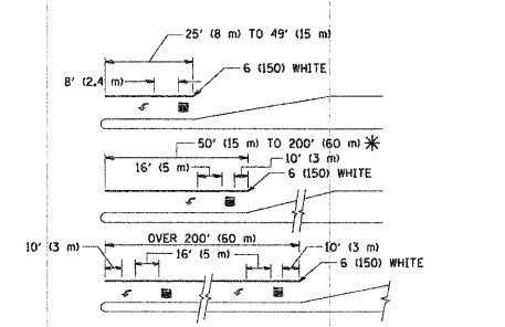
FULL SIZE LETTERS 8' (2.4 m) AND ARROWS SHALL BE USED. AREA = 15.6 SQ. FT. (1.5 m 2 ) ONLY AREA = 20.8 SQ. FT. (1.9 m 2 ) * TURN LANES IN EXCESS OF 400' (120 m) IN LENGTH MAY HAVE AN ADDITIONAL SET OF ARROW - "ONLY" INSTALLED MIDWAY BETWEEN THE OTHER TWO SETS OF ARROW - "ONLY". TYPICAL TURN LANE MARKING
