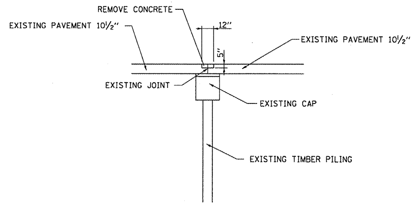
JOINT DETAIL STA. 783+70.11
