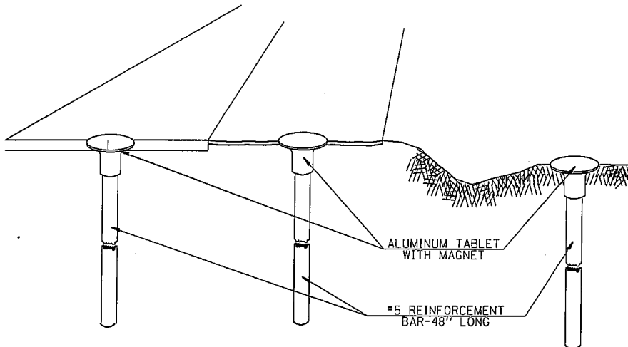
IN FLEXIBLE PAVEMENT OR SHOULDER
