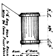
ROLLERS
