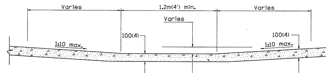
SEC. B-B
