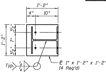
SECTION C-C
