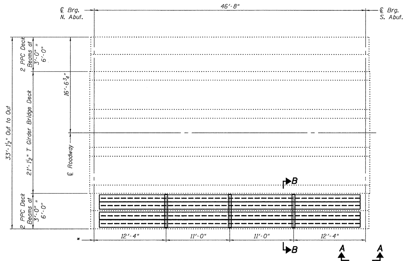
PLAN
