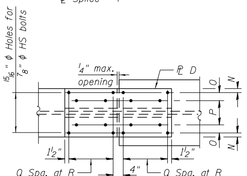
FIELD SPLICE DETAIL (SPLICE 6) (15 Required)
