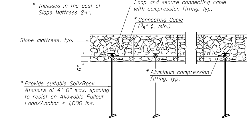
SLOPE MATTRESS SECURING DETAIL
