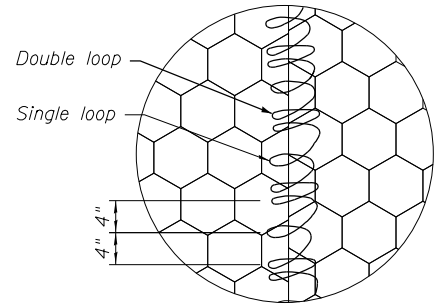
LACING DETAIL
