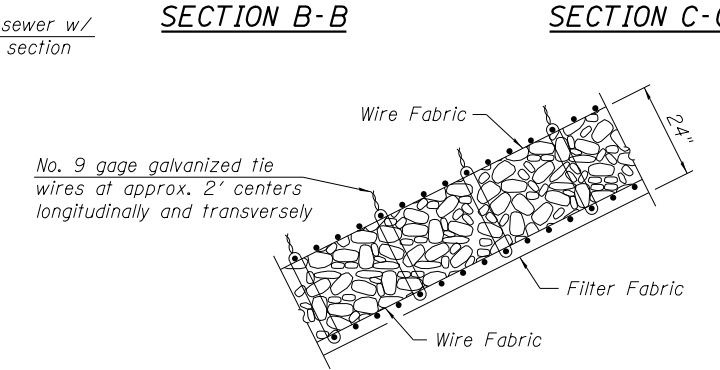
SLOPE MATTRESS DETAIL
