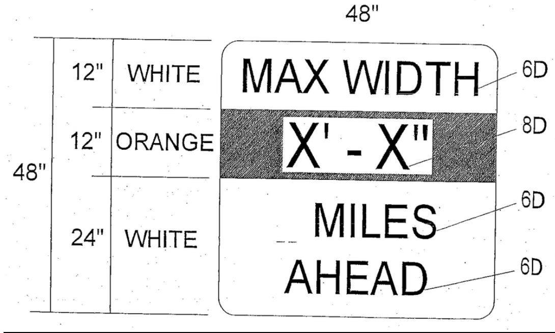
SIGN PANEL W12 - I 103 (48) MAXIMUM WIDTH SIGN
