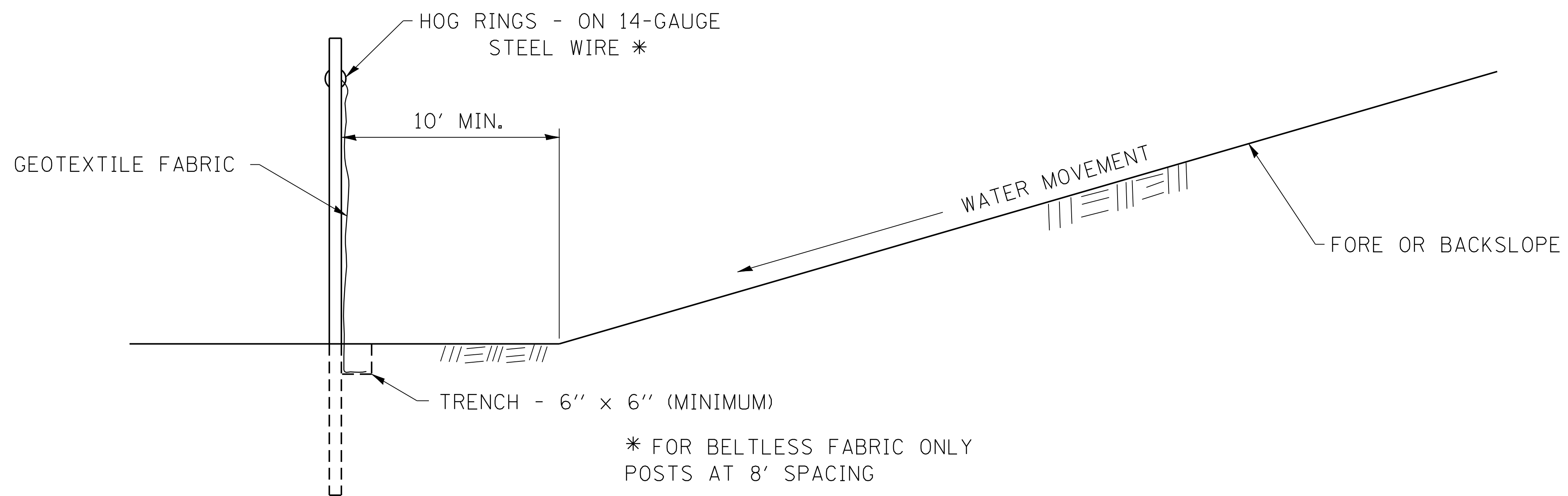
DETAILS OF SILT FENCE
