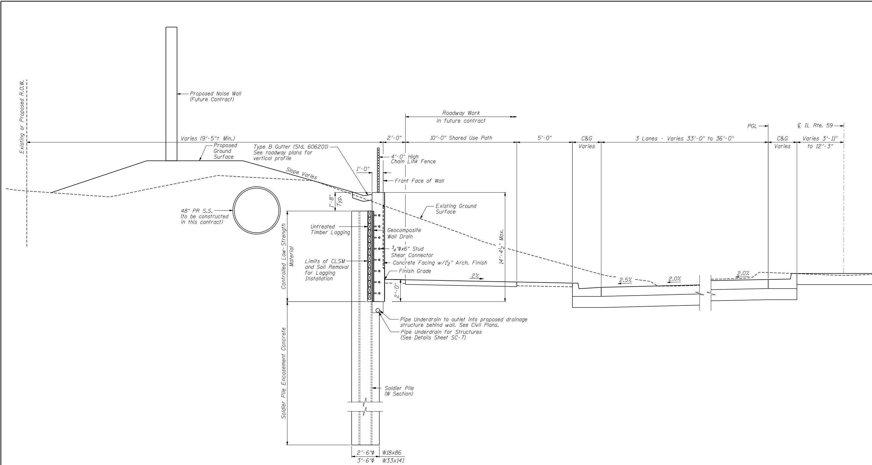
TYPICAL WALL SECTION Sta. 3965+22.00 to Sta. 3971+00 (Looking North)
