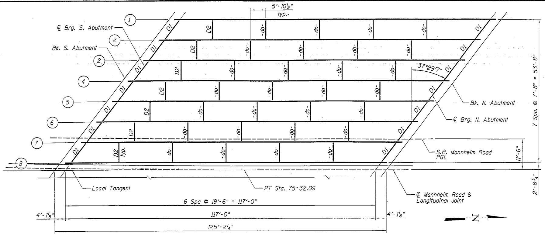
FRAMING PLAN
