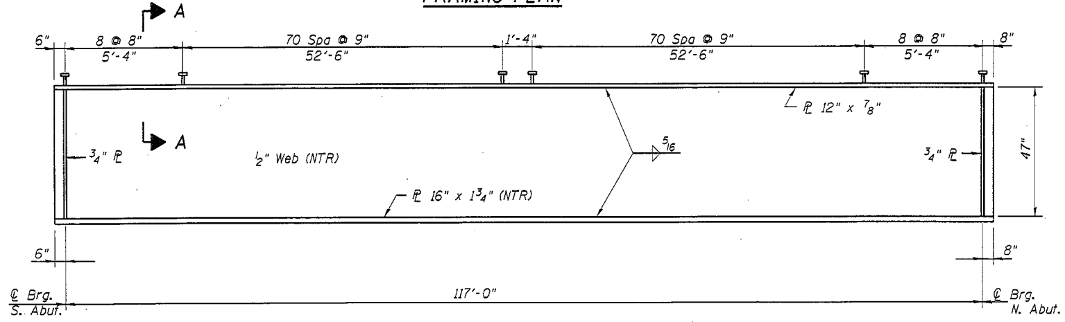
GIRDER ELEVATION
