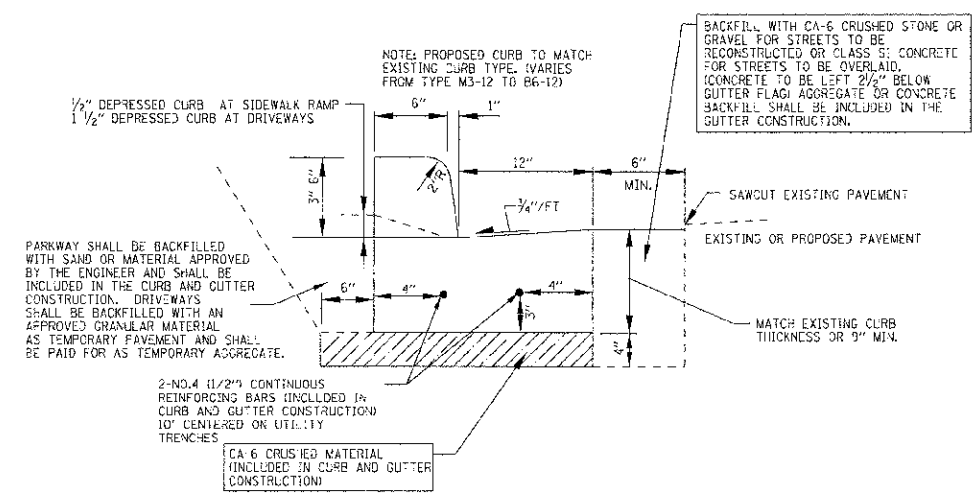
COMBINATION CONCRETE CURB AND GUTTER REMOVAL AND REPLACEMENT (NOT TO SCALE)
