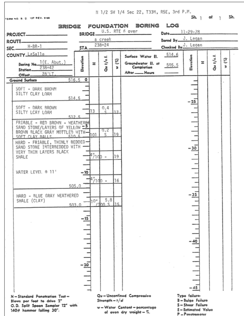
BORING B-1 (1978)
