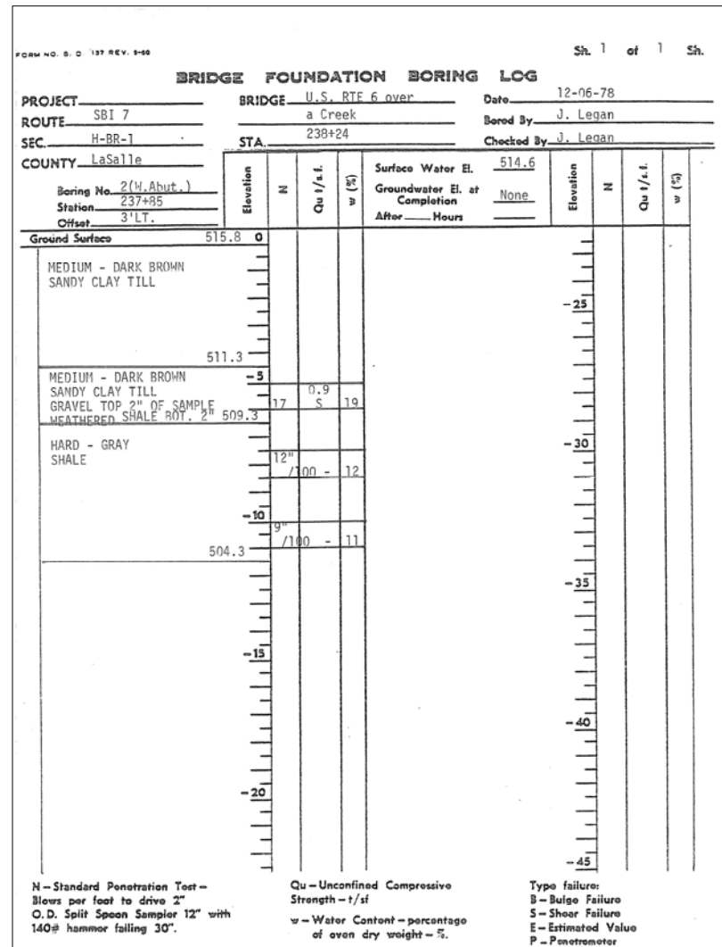
BORING B-2 (1978)
