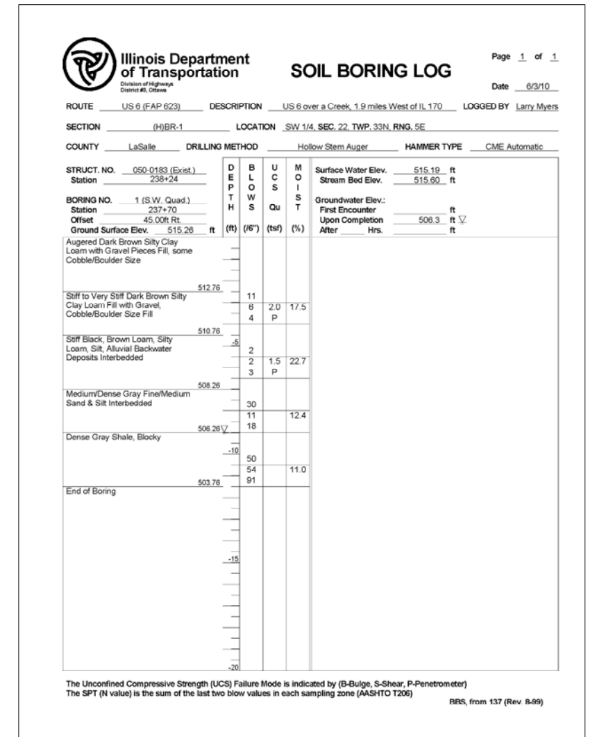
BORING B-1 (2010)
