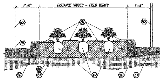
2 SECTION THRU NEW STREETSCAPE IMPROVEMENTS C3.1 1' 6\"/>
