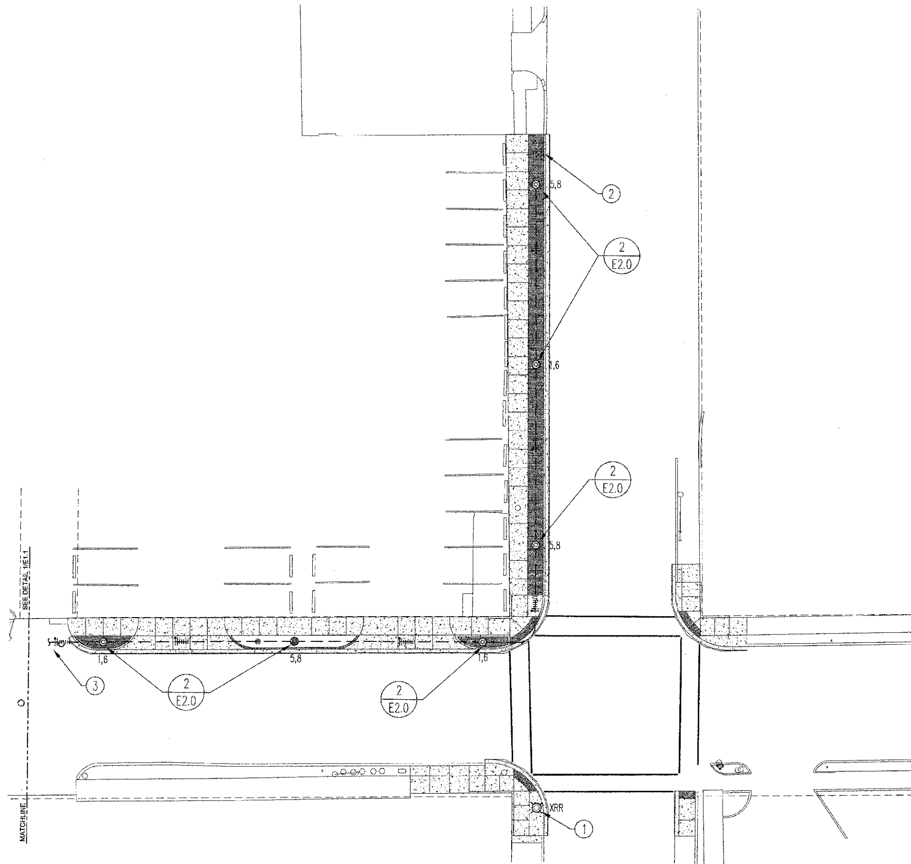
① LARGE SCALE ELECTRICAL LAYOUT PLAN - WASHINGTON AND NORTH MAIN STREETS E1.2 SCALE: 1"=10'-0"
