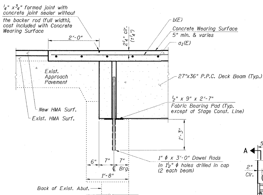
SECTION THRU ABUTMENT @ ROADWAY
